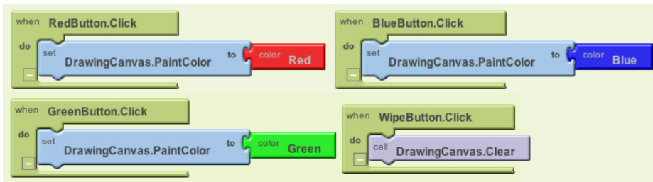
Figure 2-14. Clicking the color buttons changes the canvas's PaintColor; clicking Wipe clears the screen
